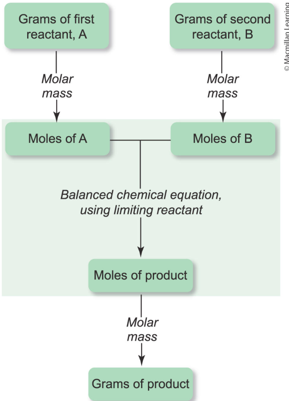
FIGURE 5.7 Procedure for Limiting-Reactant Problems Involving Masses
